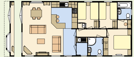
Optional bay window 40 x 20 – 3 bedroom/8 berth
