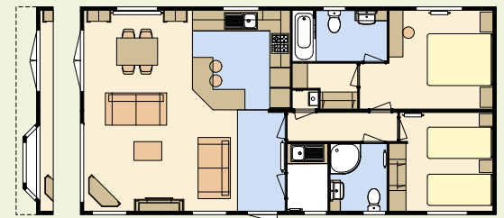
Optional bay window 40 x 20 – 2 bedroom/6 berth
